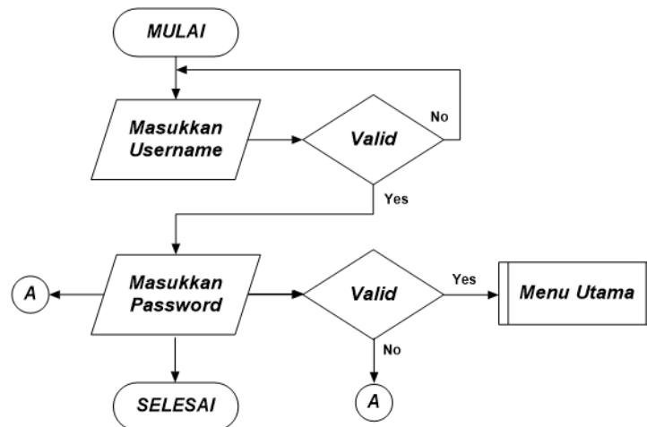
Gambar 4.2 Flowchart Halaman Login
