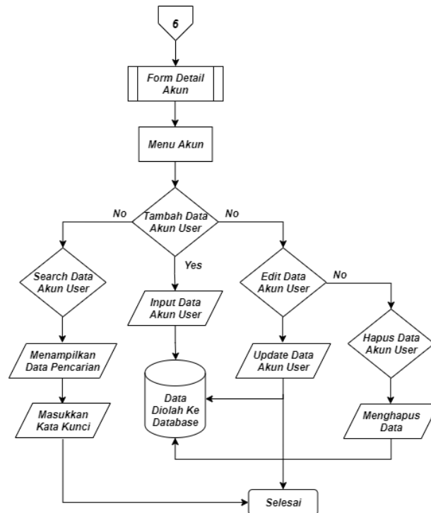
Gambar 4.7 Flowchart Halaman Akun
