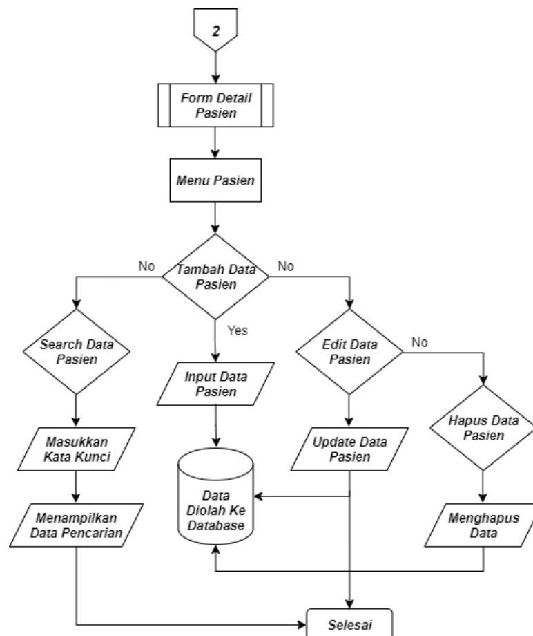
Gambar 4.3 Flowchart Halaman Pasien
