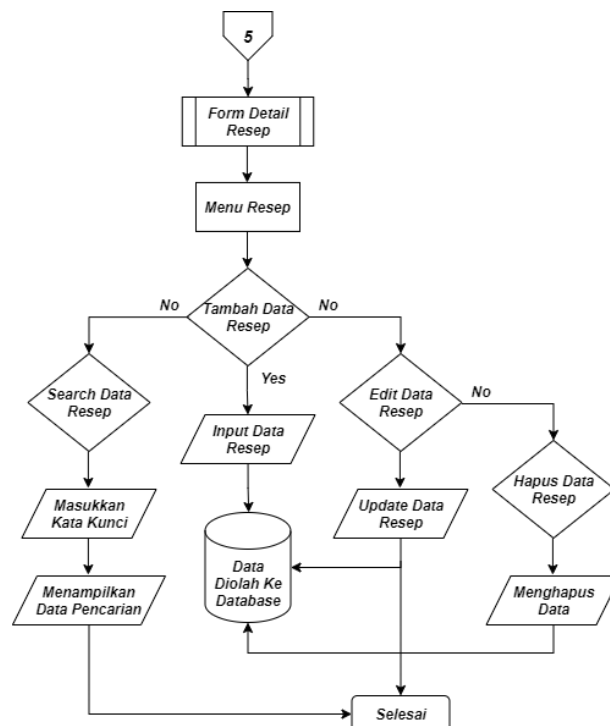
Gambar 4.6 Flowchart Halaman Resep
