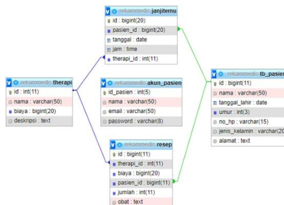
Gambar 4.7 ERD (Entity Rational Diagram)
