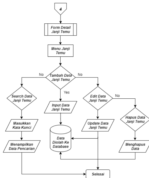
Gambar 4.5 Flowchart Halaman Janji Temu
